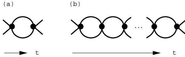
Figure A1. Singular diagrams contributing to the finite-size free energy \Delta\mathcal{C}_p(u_0) in the expansion (A.3). The lines denote unperturbed single-line propagators \langle \phi(r_1, t_{01})\phi(r_2, t_{02}) \rangle , the dots pair contact vertices \Phi_2(t_0) . (a) A one-loop diagram containing a primitive pole in y_0 . (b) An N -loop diagram containing a pole in y_0 of order N - 1 .
